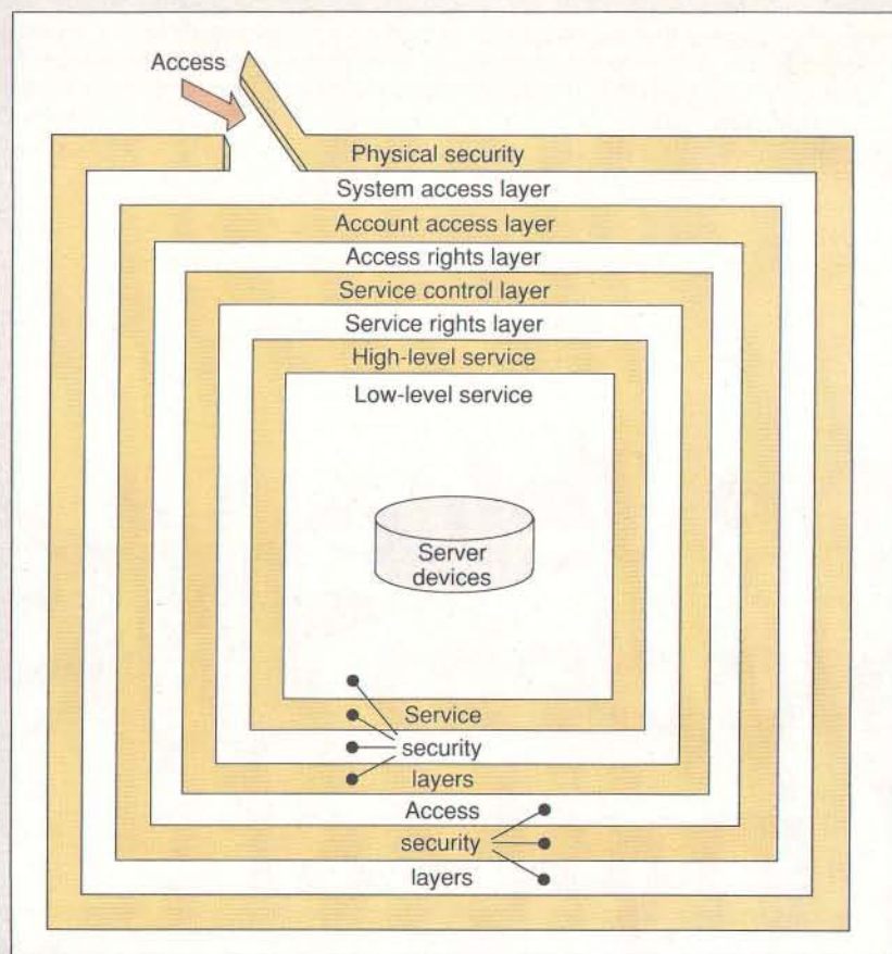
Figure A: Like an onion, good security is composed of layers wrapped on layers. In the file-server model, access to the actual device must go through three layers of access security and four layers of service security.
